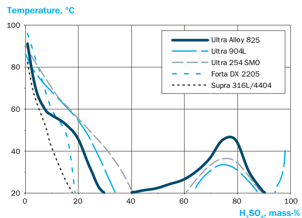
Fig. 2. Isocorrosion diagram in naturally aerated sulfuric acid of chemical purity with an addition of 200 ppm chlorides, based on uniform corrosion tests with sample activation according to ISO 18069. The line represents a limit for corrosion resistance below which the corrosion rate is lower than 0.1 mm/year.
