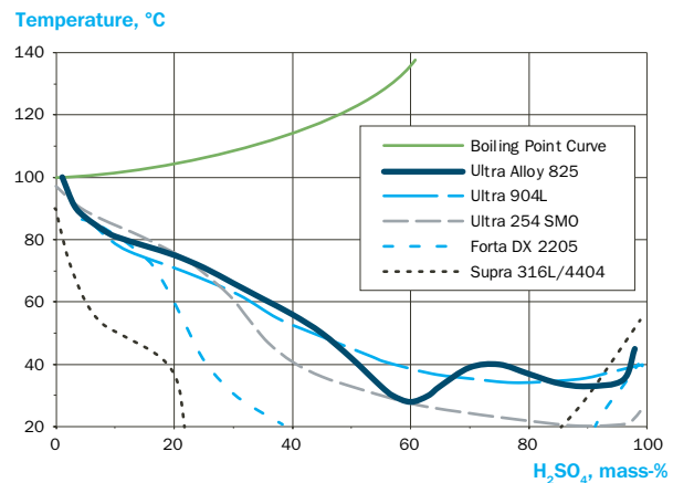
Fig. 1. Isocorrosion diagram in naturally aerated sulfuric acid of chemical purity, based on uniform corrosion tests with sample activation according to ISO 18069. The line represents a limit for corrosion resistance below which the corrosion rate is lower than 0.1 mm/year.
