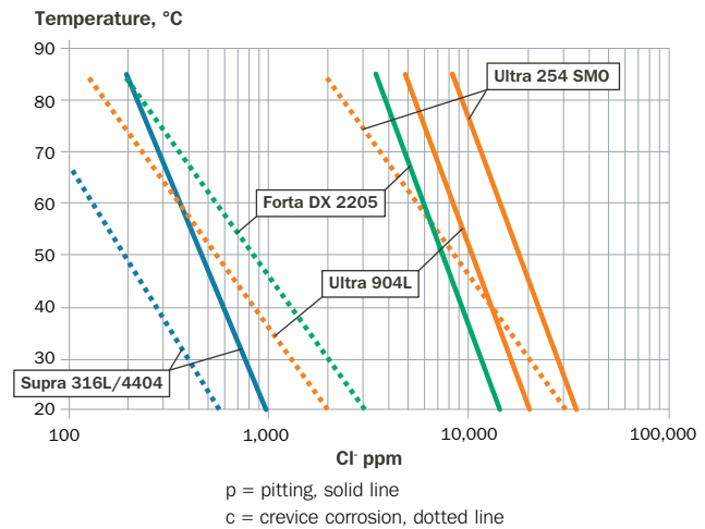
Fig. 10. Engineering diagram indicating the maximum temperature and chloride concentration allowed in slightly chlorinated (< 1 ppm) waters.
