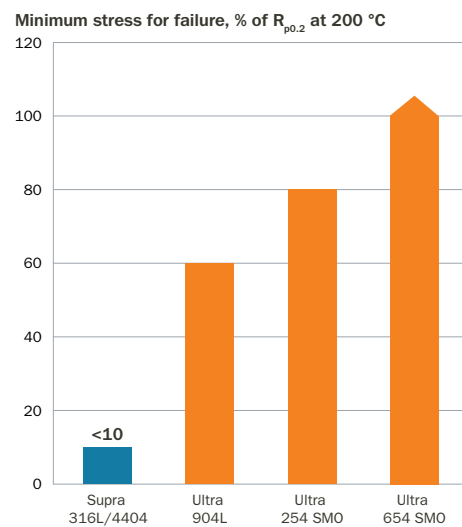
Fig. 11. Typical threshold stresses determined using the drop evaporation test.
